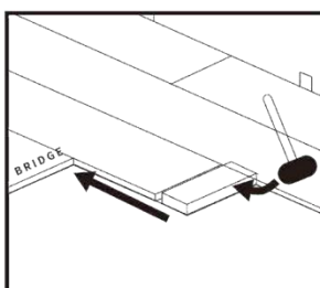
Step 7: Tap end of plank with hammer and tapping block to lock ends of planks together. Remove support bridge and continue with this method until you have completed installing the row. Note: BE SURE TO TAP ON EDGE OF VINYL SO AS NOT TO DAMAGE LOCKING PROFILE.
